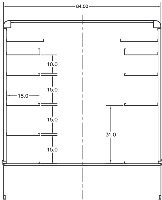
CROSS SECTION BAY #1
